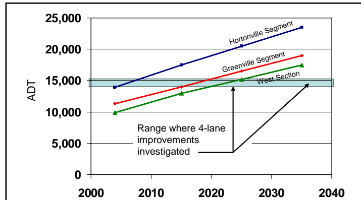
Figure 1.3-1 WIS 15 Projected Traffic Volumes
